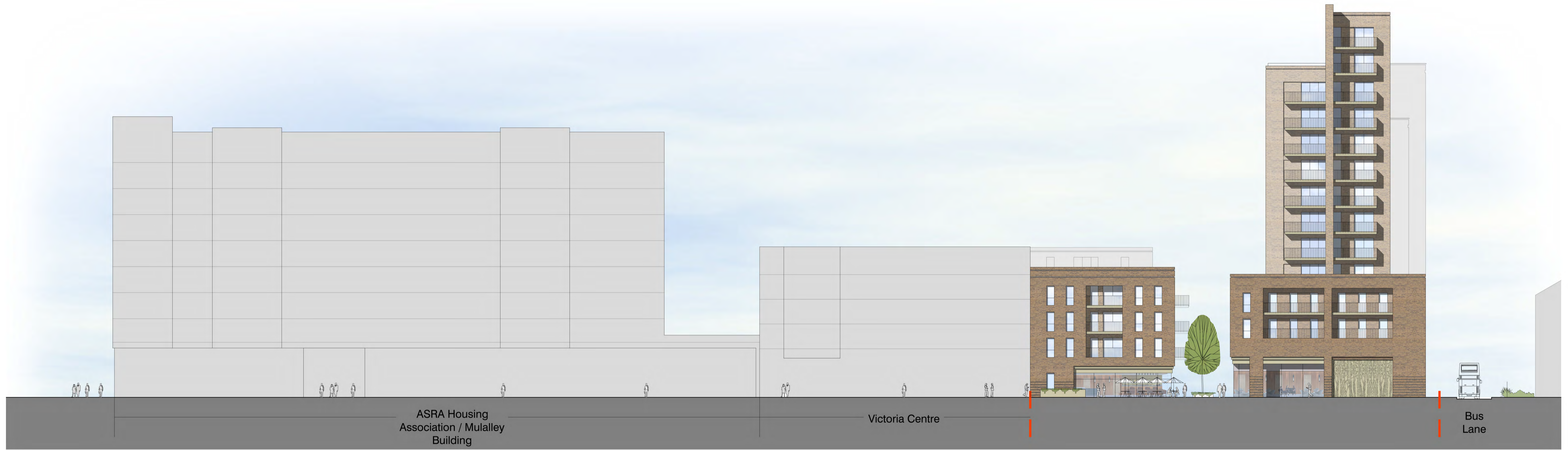
A-A - Front Elevation
